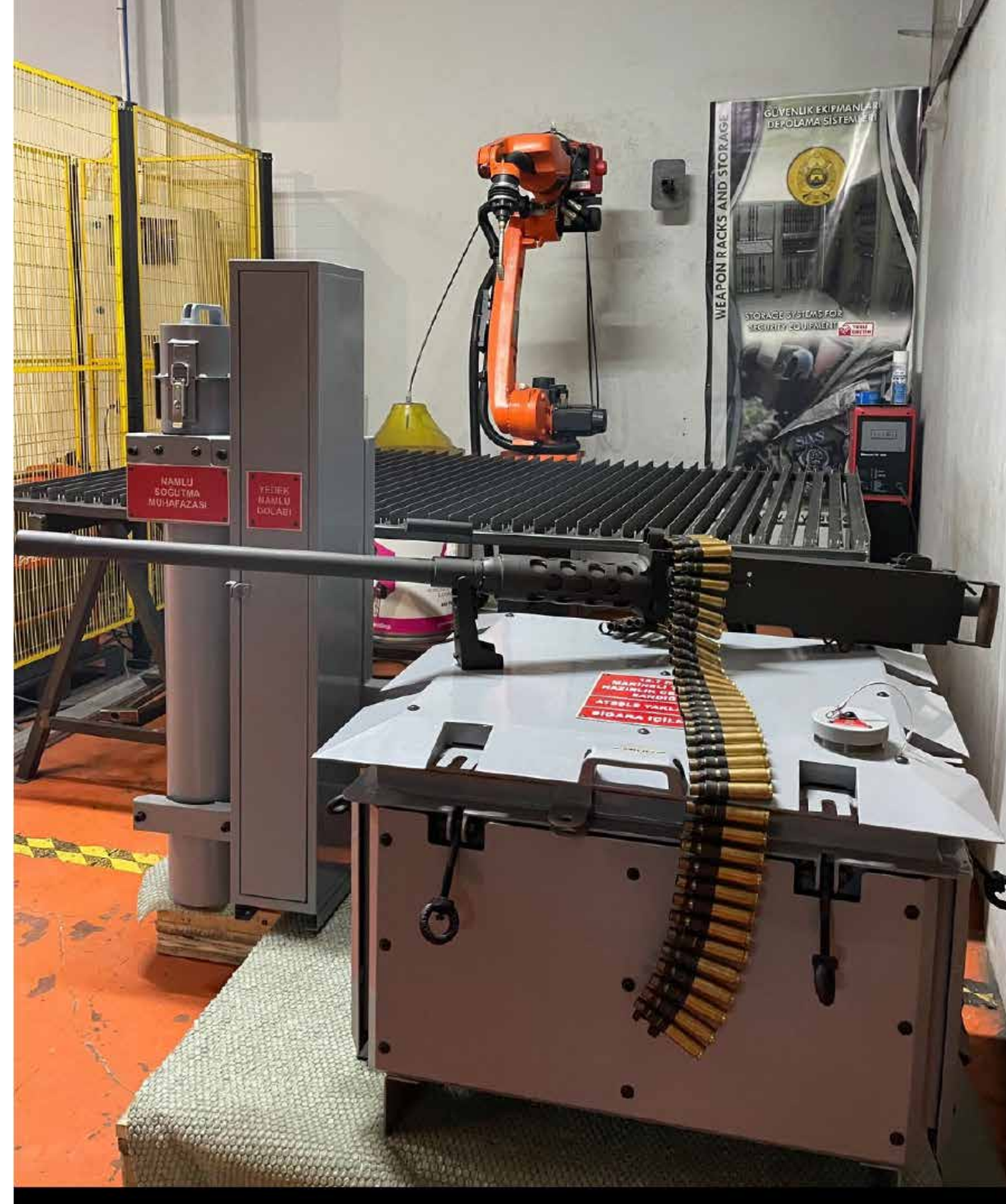
REMOTE-CONTROLLED WEAPON CONSOLES AND READY USE AMMUNITION LOCKERS FOR THE TCG AKHİSAR AND TCG KOÇHİSAR WAR SHIP, TO BE DELIVERED TO THE TURKISH NAVY
